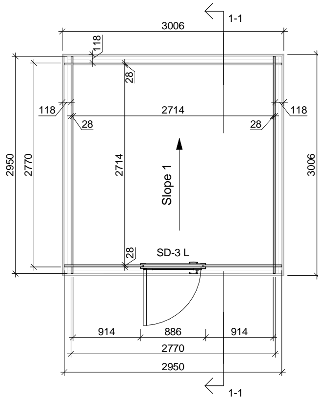
FLOOR PLAN
