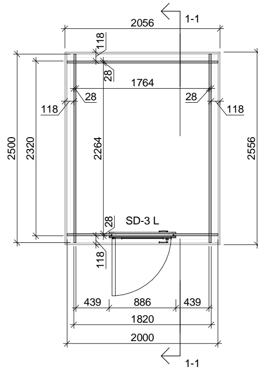
FLOOR PLAN
