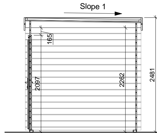
SECTION 1-1
