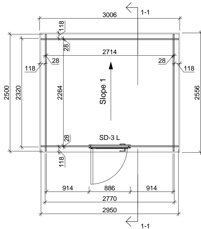
FLOOR PLAN
