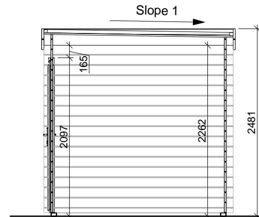
SECTION 1-1
