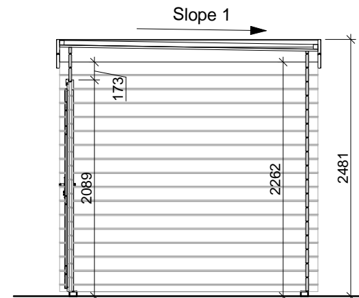
SECTION 1-1
