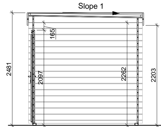
SECTION 1-1
