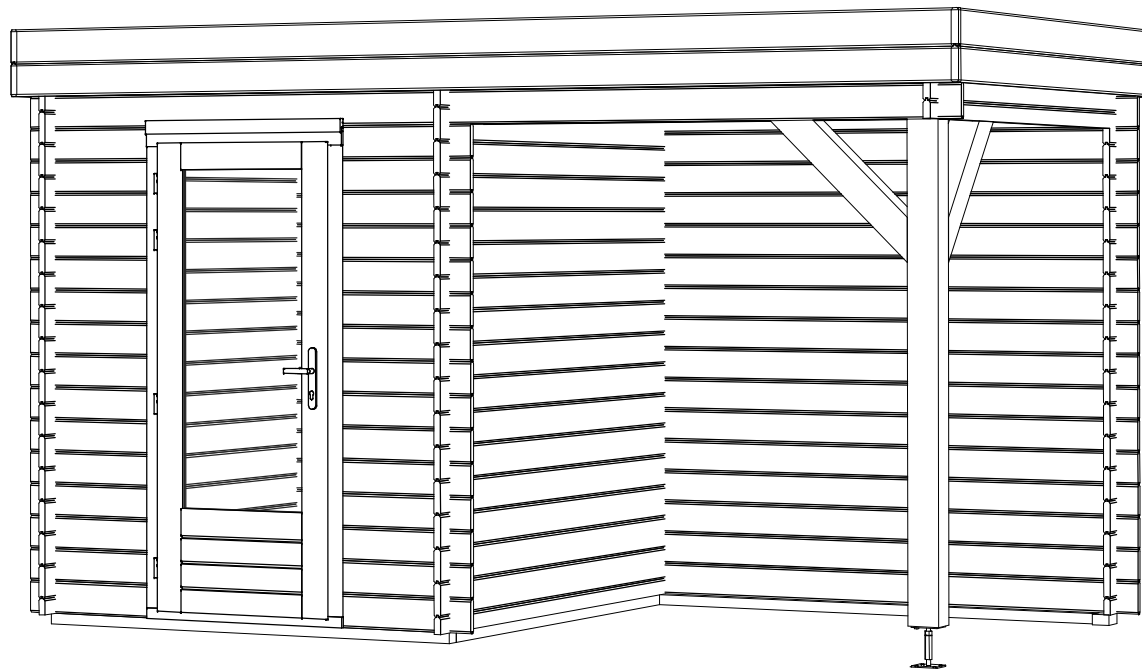
3D VIEW
